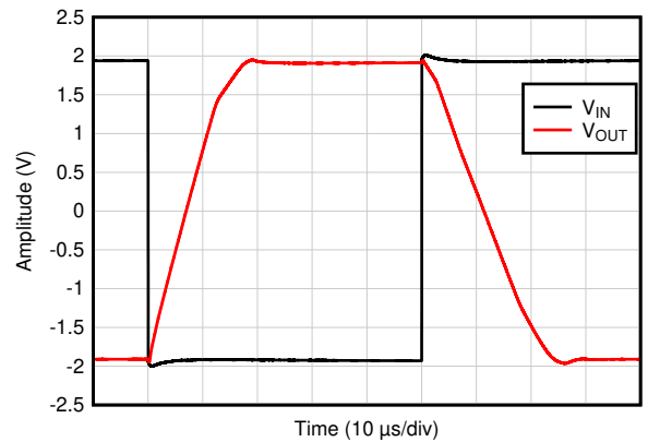
Figure 7-38. Large-Signal Step Response
