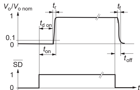
Fig. 6 Typical output response to the SD-signal
