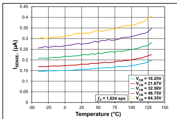
FIGURE 2-27: I_{SENSE-} vs. T_A , f_S = 1,024 sps, Common Mode, Multiple V_{CM} .
