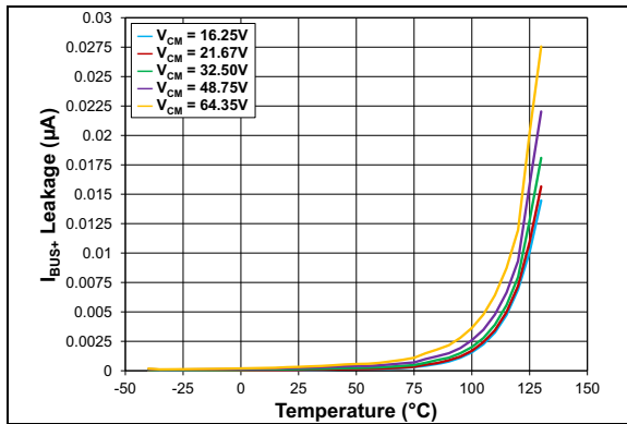
FIGURE 2-32: V_{BUS+} Leakage Current vs. T_A , Common Mode, Multiple V_{CM} .
