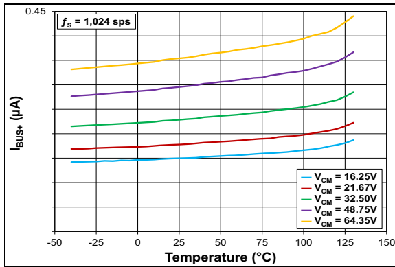
FIGURE 2-31: I_{BUS+} vs. T_A , Common Mode, Multiple V_{CM} .
