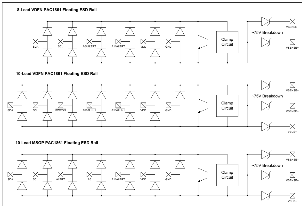
FIGURE 1-1: PAC1861 ESD Protection Circuitry.
