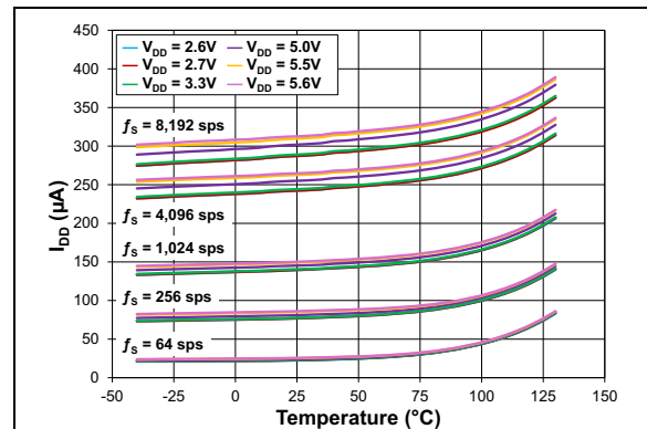
FIGURE 2-24: I_{DD} vs. T_A , Multiple V_{DD} , Multiple f_S .
