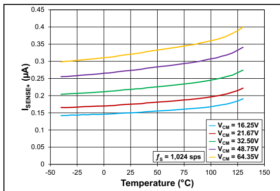
FIGURE 2-28: I_{SENSE+} vs. T_A , Common Mode, Multiple V_{CM} .
