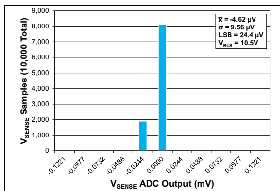
FIGURE 2-17: V_{SENSE} Zero Input Histogram, Bipolar FSR/2 Mode, \pm 50\text{ mV} Range, n = 10,000 Total Samples, 8x Average.
