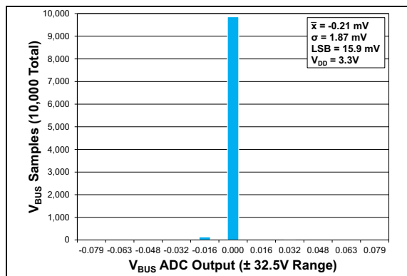
FIGURE 2-18: V_{BUS} Zero Input Histogram, Bipolar FSR/2 Mode, \pm 32.5\text{V} Range, n = 10,000 Total Samples, 8x Average.
