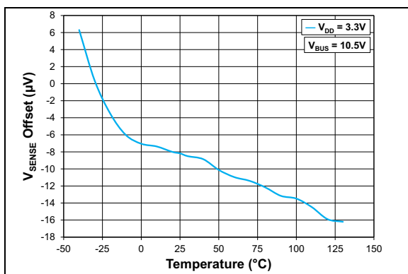
FIGURE 2-20: V_{SENSE} Offset vs. T_A , V_{DD} = 3.3\text{V} , V_{BUS} = 10.5\text{V} , Bipolar FSR Mode.
