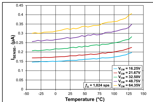
FIGURE 2-27: I_{SENSE-} vs. T_A , Common Mode, Multiple V_{CM} .
