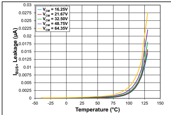
FIGURE 2-32: V_{BUS+} Pin Input Current Leakage vs. Temperature, Multiple V_{CM} .
