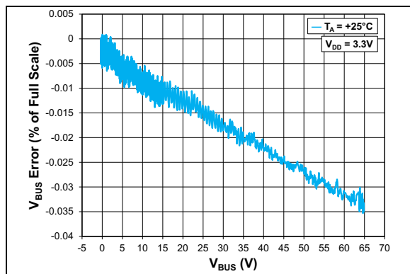
FIGURE 2-15: V_{BUS} Error vs. V_{BUS} , V_{DD} = 3.3\text{V} , T_A = +25^\circ\text{C} , Bipolar FSR Mode, Zoom View.
