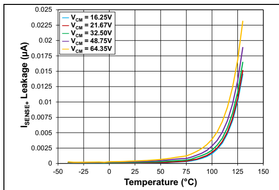
FIGURE 2-30: I_{SENSE+} Leakage Current vs. T_A , Common Mode, Multiple V_{CM} .
