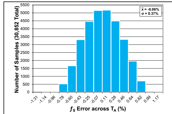
FIGURE 2-34: Sample Rate ( f_S ) Error across T_A = -40^{\circ}\text{C} to +125^{\circ}\text{C} , n = 30,852 Total Samples.
