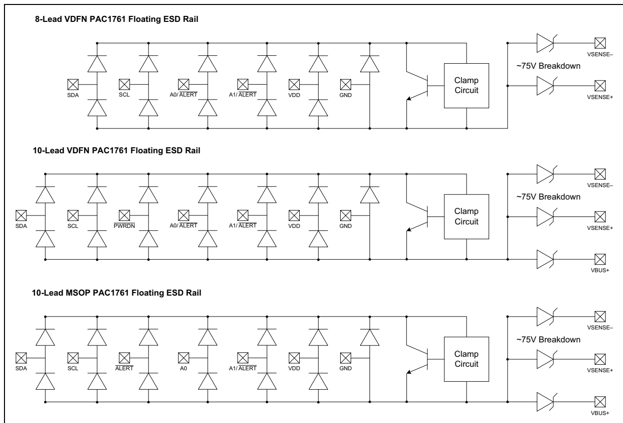
FIGURE 1-1: PAC1761 ESD Protection Circuitry.
