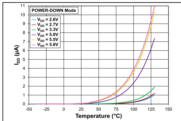
FIGURE 2-26: I_{DD} in Power-down Mode vs. T_A , Multiple V_{DD} . (10-Lead VDFN only)
