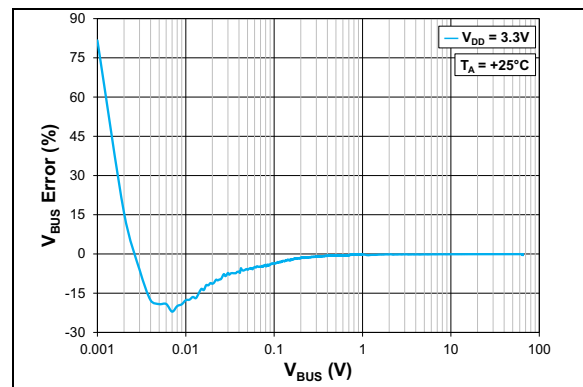
FIGURE 2-11: V_{BUS} Error vs. V_{BUS} , T_A = +25^\circ\text{C} , V_{DD} = 3.3\text{V} , Unipolar Mode, Logarithmic Scale.
