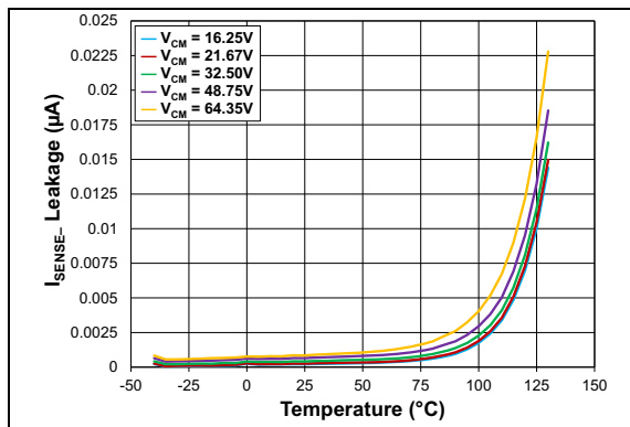
FIGURE 2-29: I_{SENSE-} Leakage Current vs. T_A , Common Mode, Multiple V_{CM} .
