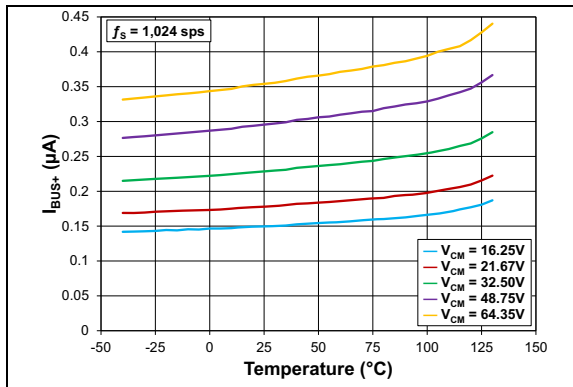
FIGURE 2-31: V_{BUS+} Pin Input Current vs. Temperature, Multiple V_{CM} .
