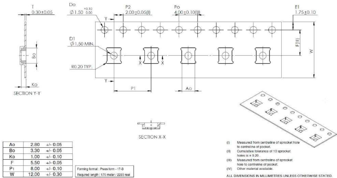
Figure 33. LGA-14L package orientation in carrier tape
