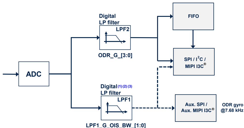
Figure 22. Gyroscope digital chain - mode 3 (OIS)
