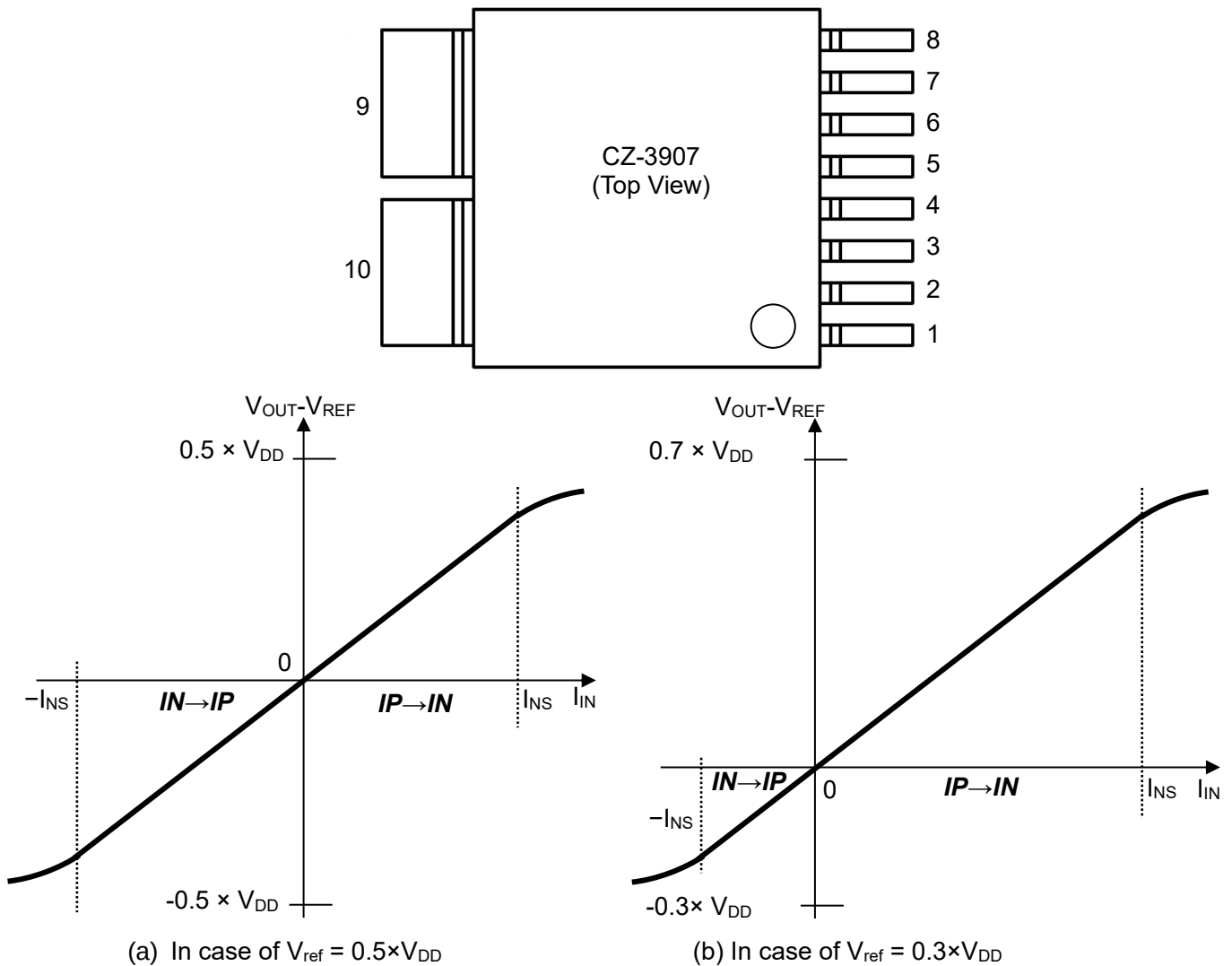
Figure 2. Pin configurations and typical output characteristics of CZ-3907
