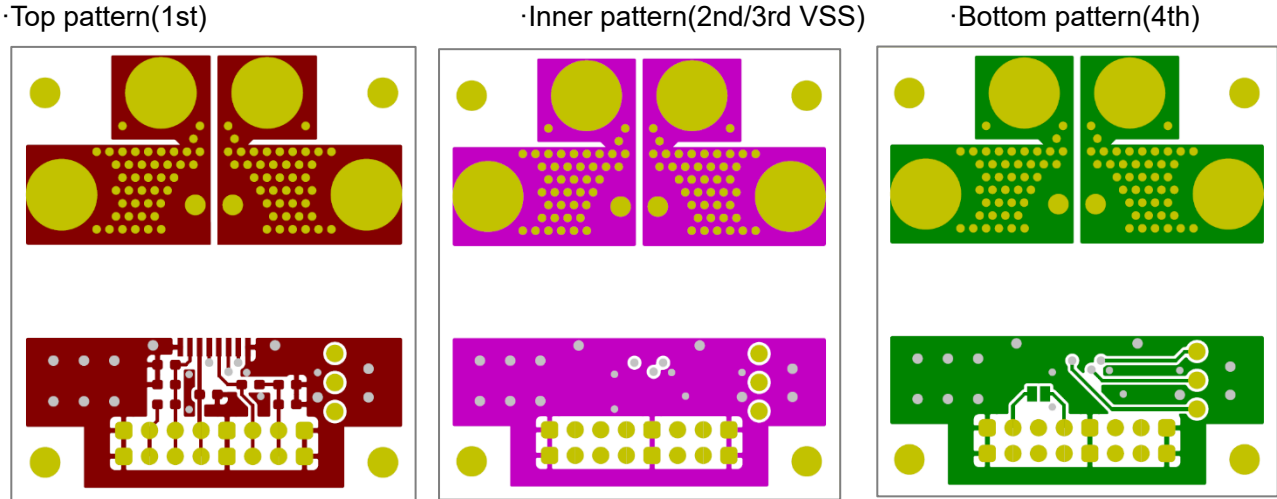
Figure 7. Board layout for measuring thermal resistance of CZ-3907
