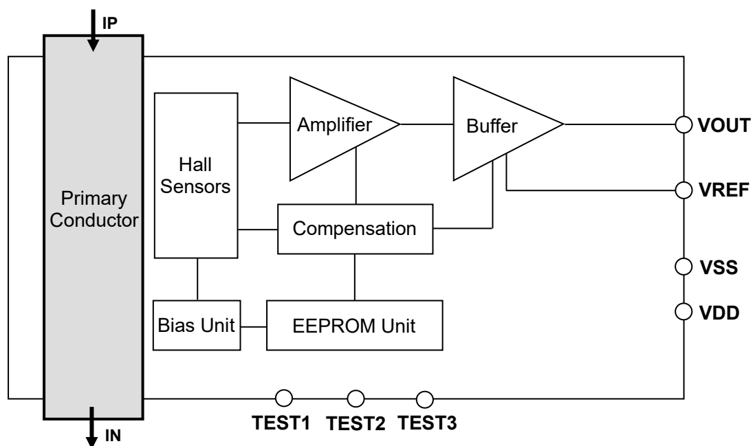
Figure 1. Block diagram of CZ-3907
