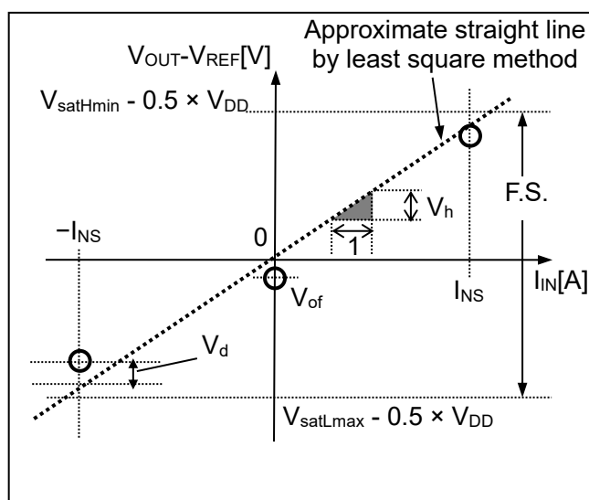
Figure 3. Output characteristics of CZ-3907
