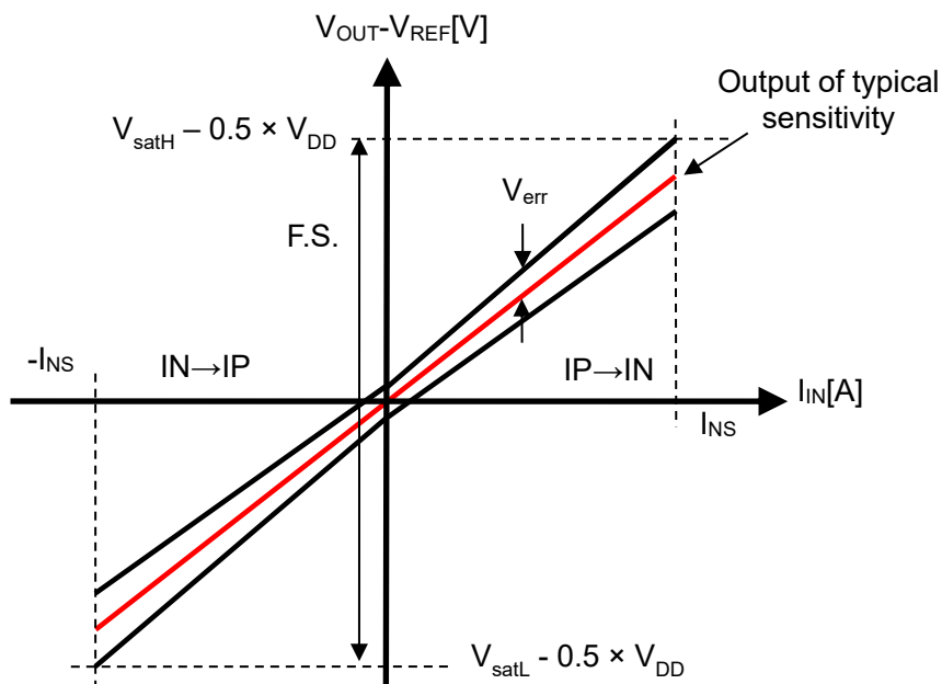
Figure 4. Total Accuracy of CZ-3907
