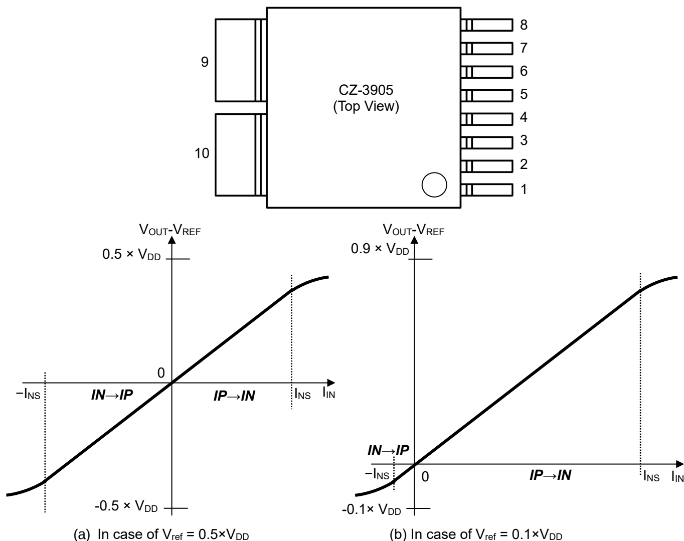
Figure 2. Pin configurations and typical output characteristics of CZ-3905
