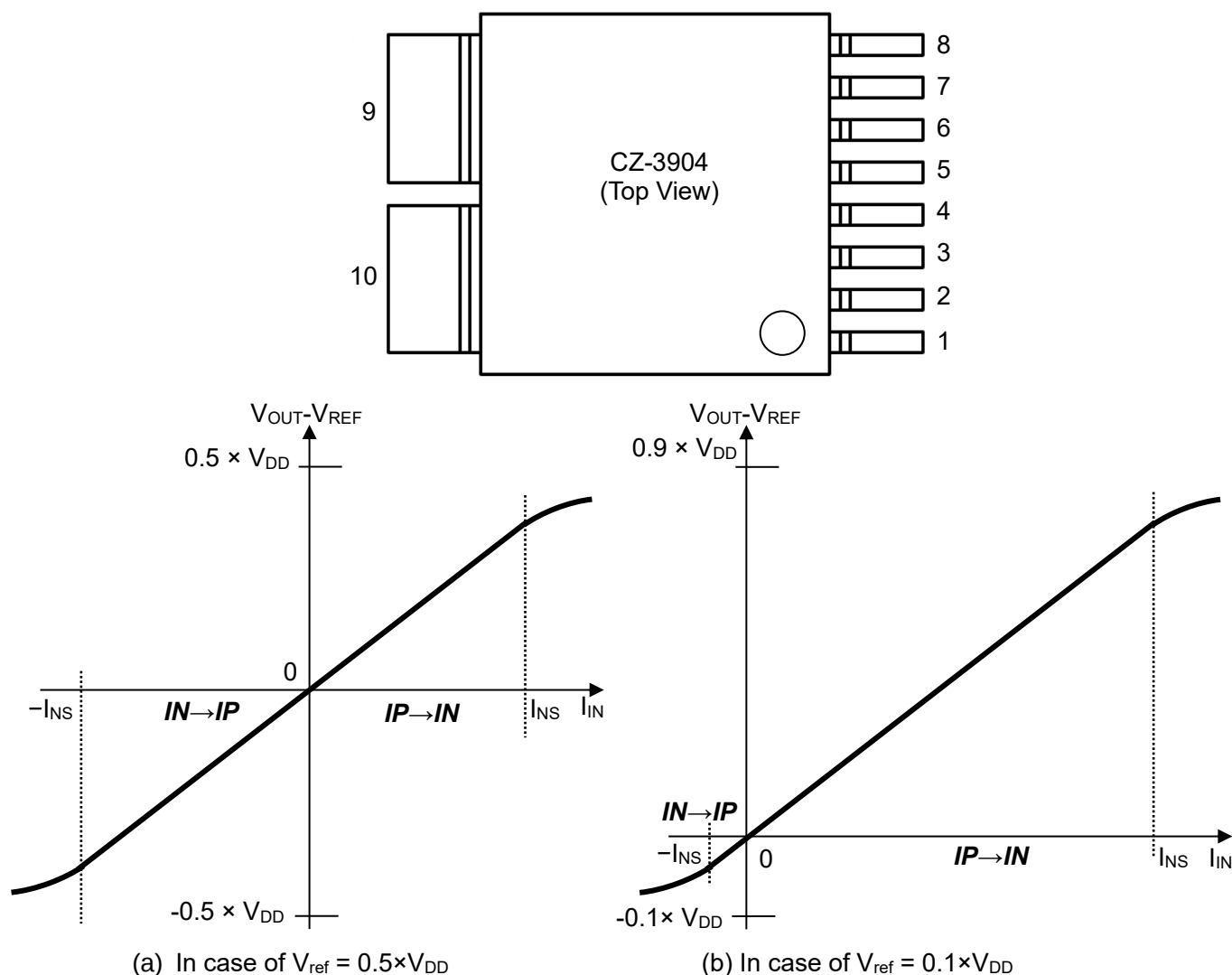
Figure 2. Pin configurations and typical output characteristics of CZ-3904
