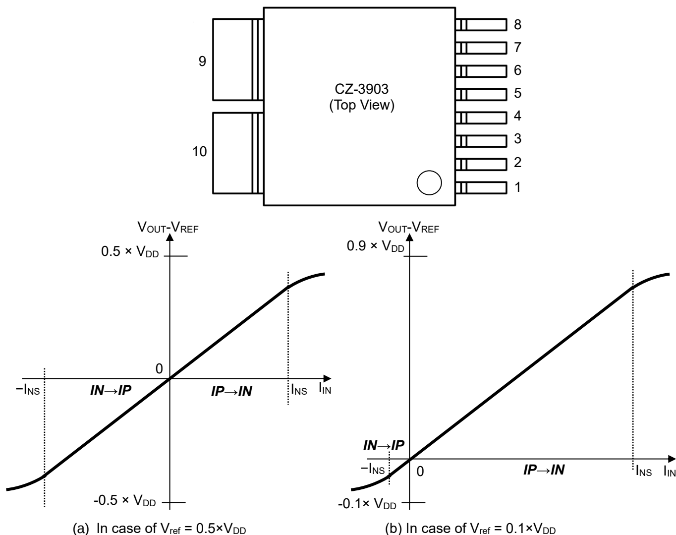
Figure 2. Pin configurations and typical output characteristics of CZ-3903
