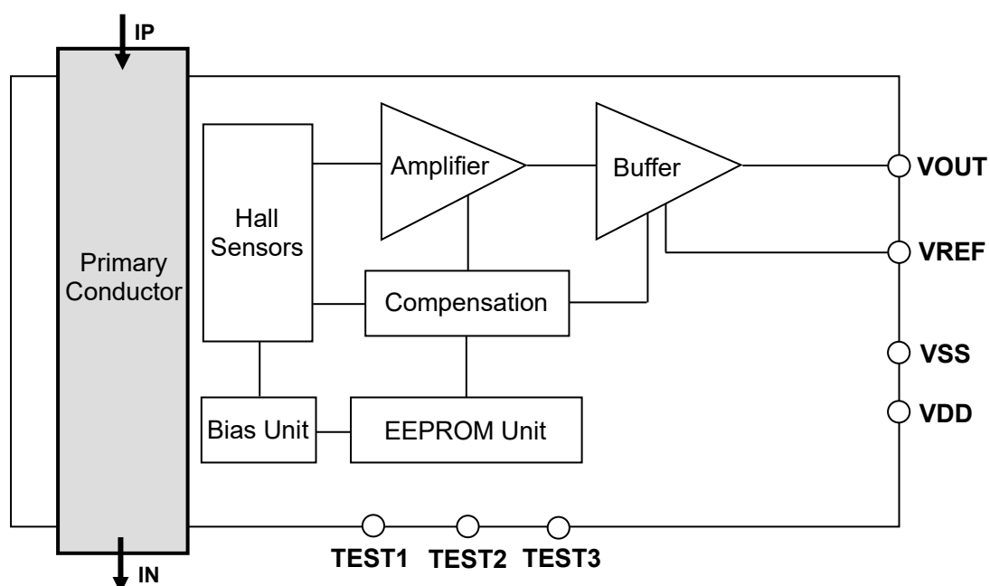
Figure 1. Block diagram of CZ-3903
