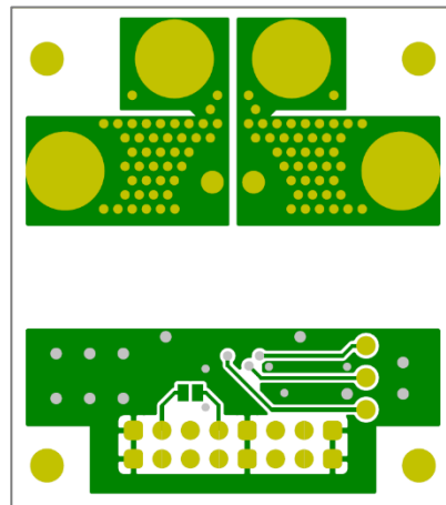
·Bottom pattern(4th)
