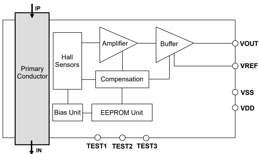
Figure 1. Block diagram of CZ-3902
