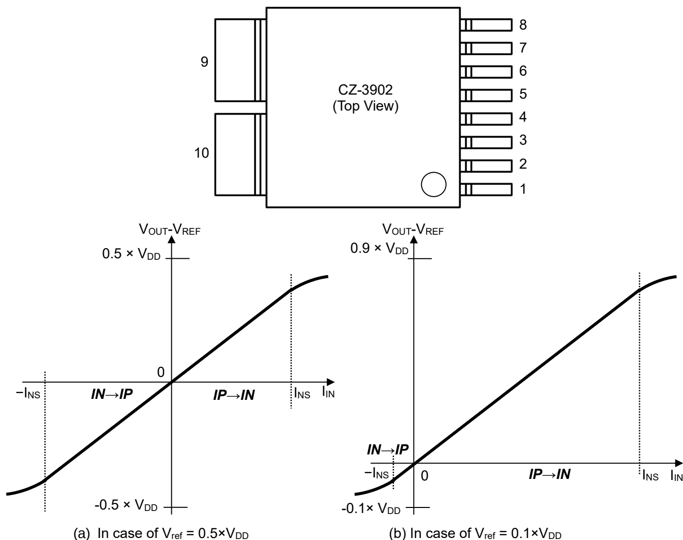
Figure 2. Pin configurations and typical output characteristics of CZ-3902
