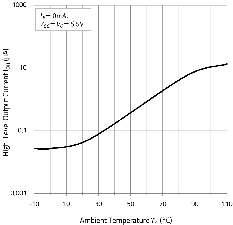
High-Level Output Current vs. Ambient Temperature:
