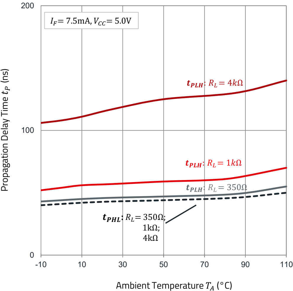
Propagation Delay Time vs. Ambient Temperature:
