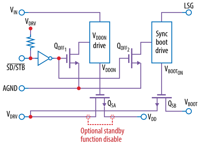
Figure 12: Simplified Circuit Diagram of V_{IN} , V_{DRV} , V_{DD} , and V_{BOOT} Power Supplies
