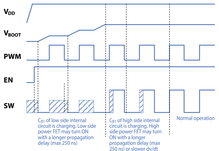
Figure 14: Behavior before complete charging of internal gate driver capacitors
