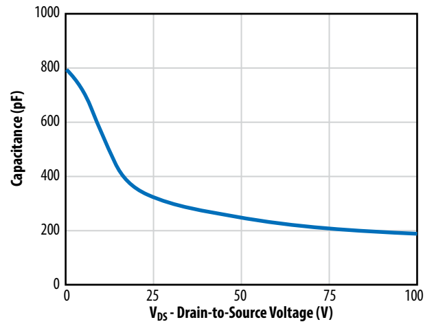
Figure 4b: C_{\text{OSS\_LSFET}} of low-side Power GaN FET
