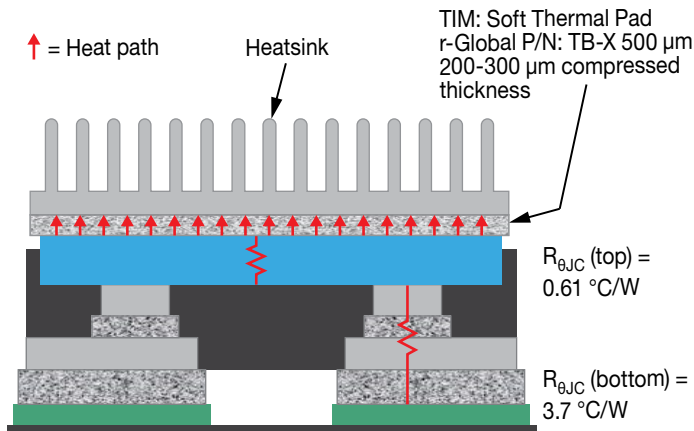
Figure 9: Parallel Thermal Resistance Paths of EPC23111 IC from Junction to Ambient
