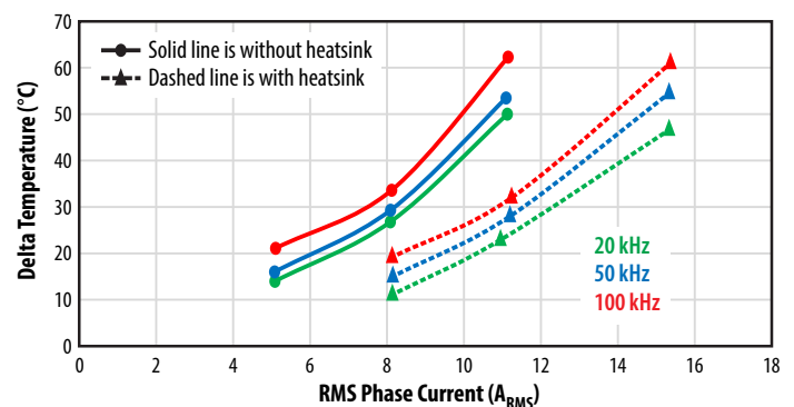
Figure 11: EPC91130 eGaN IC Temperature Increase vs. Ambient Temperature
