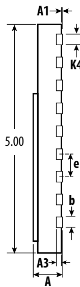
Side View 1
