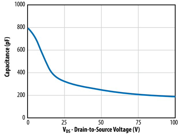
Figure 4b: C_{OSS\_LSFET} of low-side Power GaN FET
