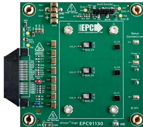
Figure 10: EPC91130 Evaluation Board (see EPC91130 Quick Start Guide for details)
