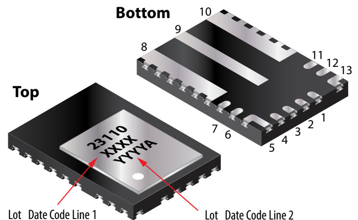
Figure 8: EPC23110 QFN package outline, pinouts and exposed backside of the GaN IC die
