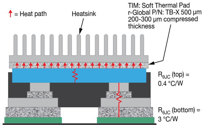
Figure 9: Parallel Thermal Resistance Paths of EPC23108 IC from Junction to Ambient
