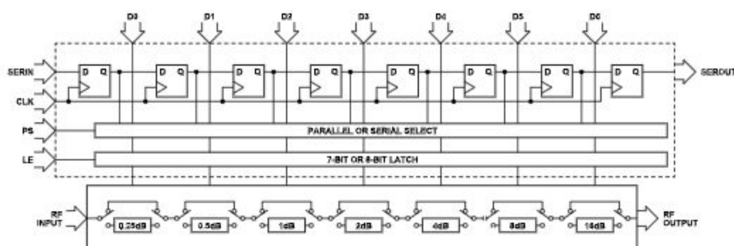
Figure 34. Simplified Circuit Diagram
