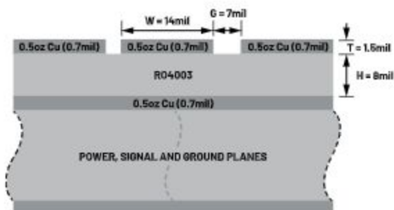
Figure 39. Example PCB Stackup
