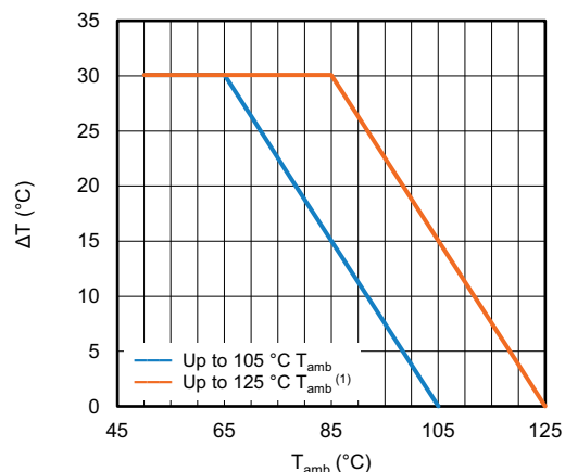
Maximum allowed component temperature rise ( \Delta T ) as function of ambient temperature ( T_{amb} )
