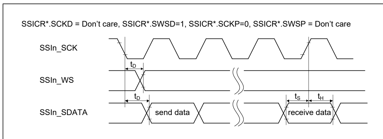
Figure 2.5-51 SSI Timing (2)
