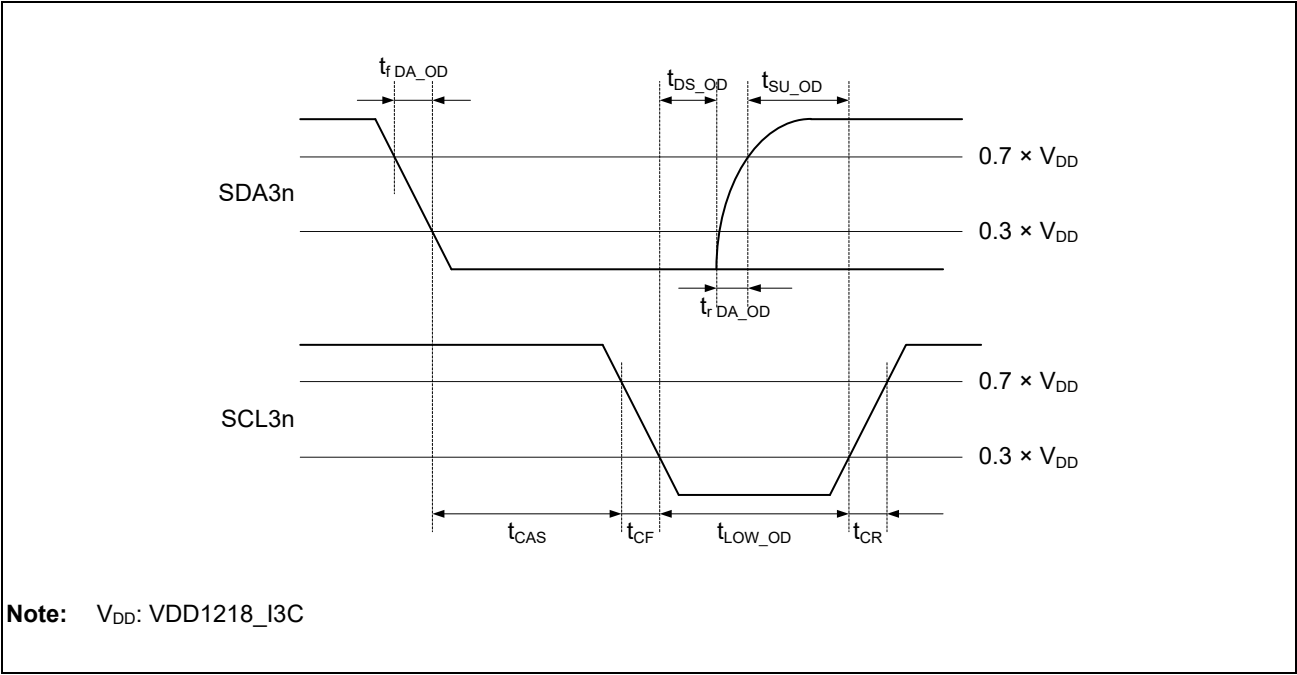
Figure 2.5-40 I3C START Condition Timing
