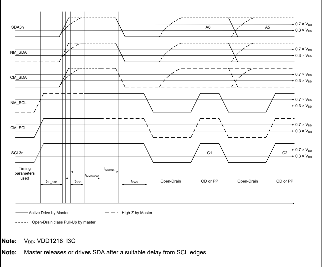
Figure 2.5-46 I3C Timing
