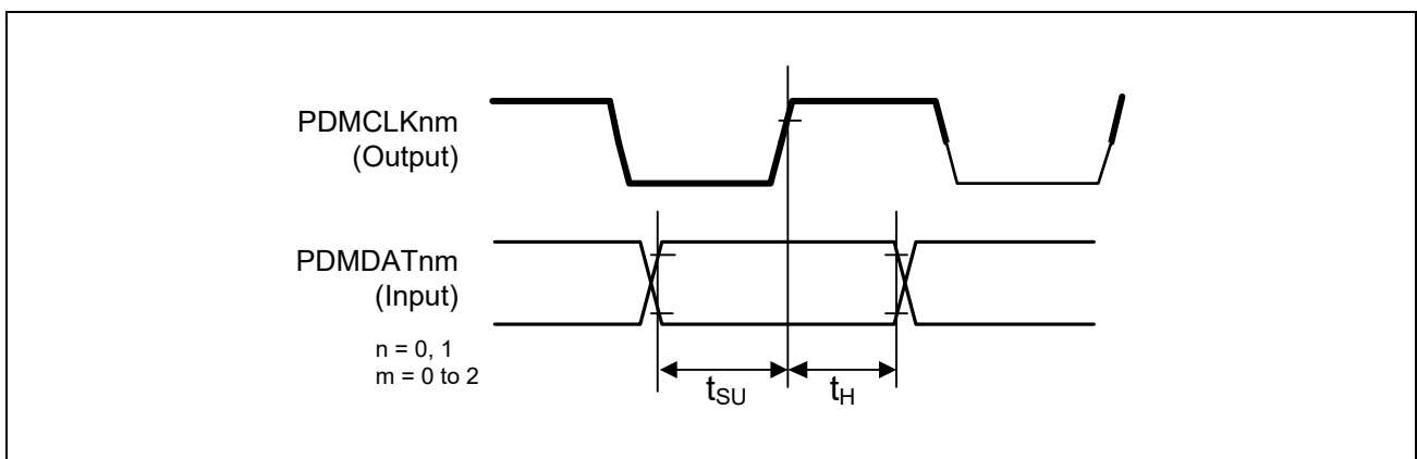
Figure 2.5-55 Timing of Clock Output (Synchronized with the rise of PDMCLKnm)
