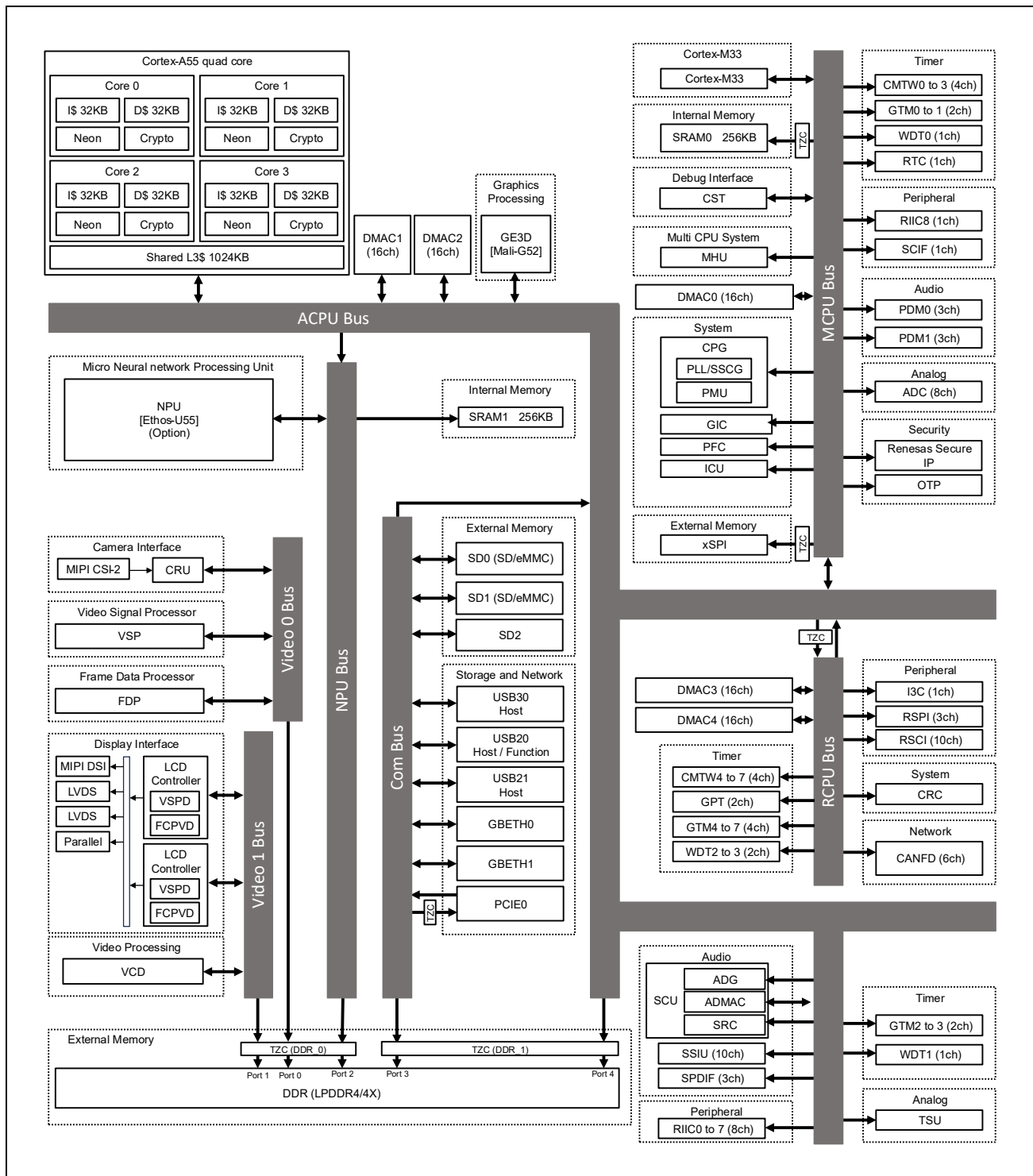
Figure 1.3-1 Block Diagram
