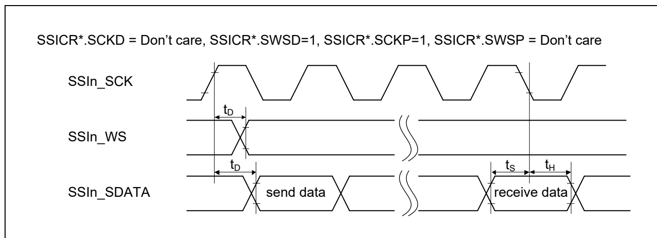
Figure 2.5-50 SSI Timing (1)
