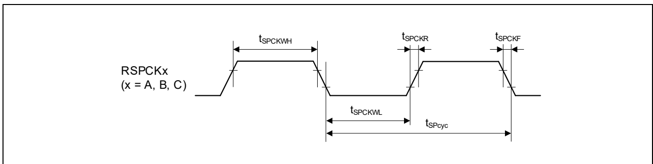
Figure 2.5-28 RSPI Clock Timing
