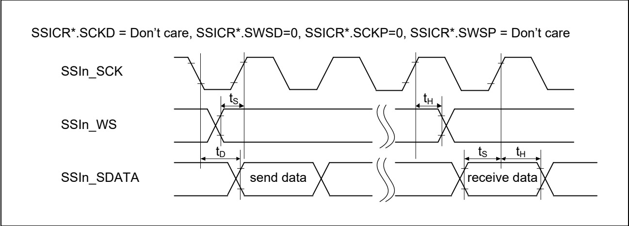
Figure 2.5-53 SSI Timing (4)
