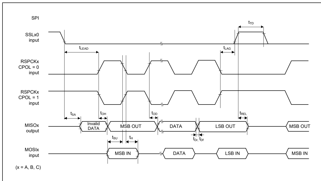
Figure 2.5-32 RSPI Timing (Slave, Motorola RSPI, CPHA = 1)
