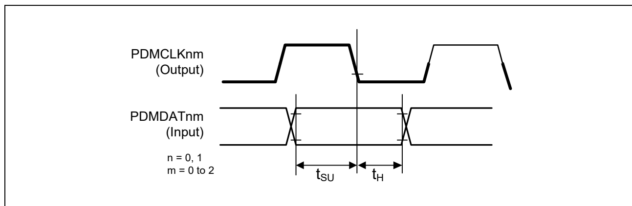
Figure 2.5-56 Timing of Clock Output (Synchronized with the fall of PDMCLKnm)
