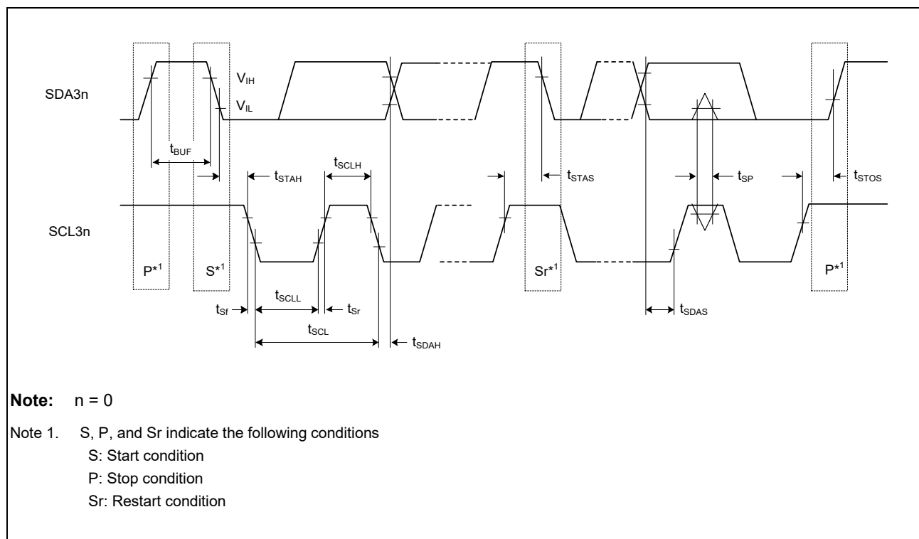
Figure 2.5-37 I3C Bus Interface Input/Output Timing
