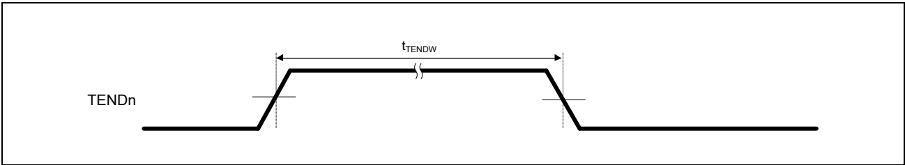
Figure 2.5-8 DMAC TENDn Timing
