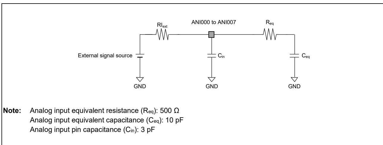
Figure 2.6-1 A/D Converter Equivalent Circuit and Peripheral Configuration Diagram
