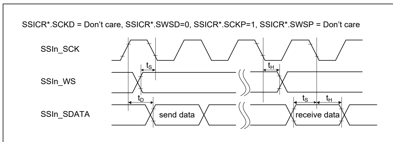
Figure 2.5-52 SSI Timing (3)
