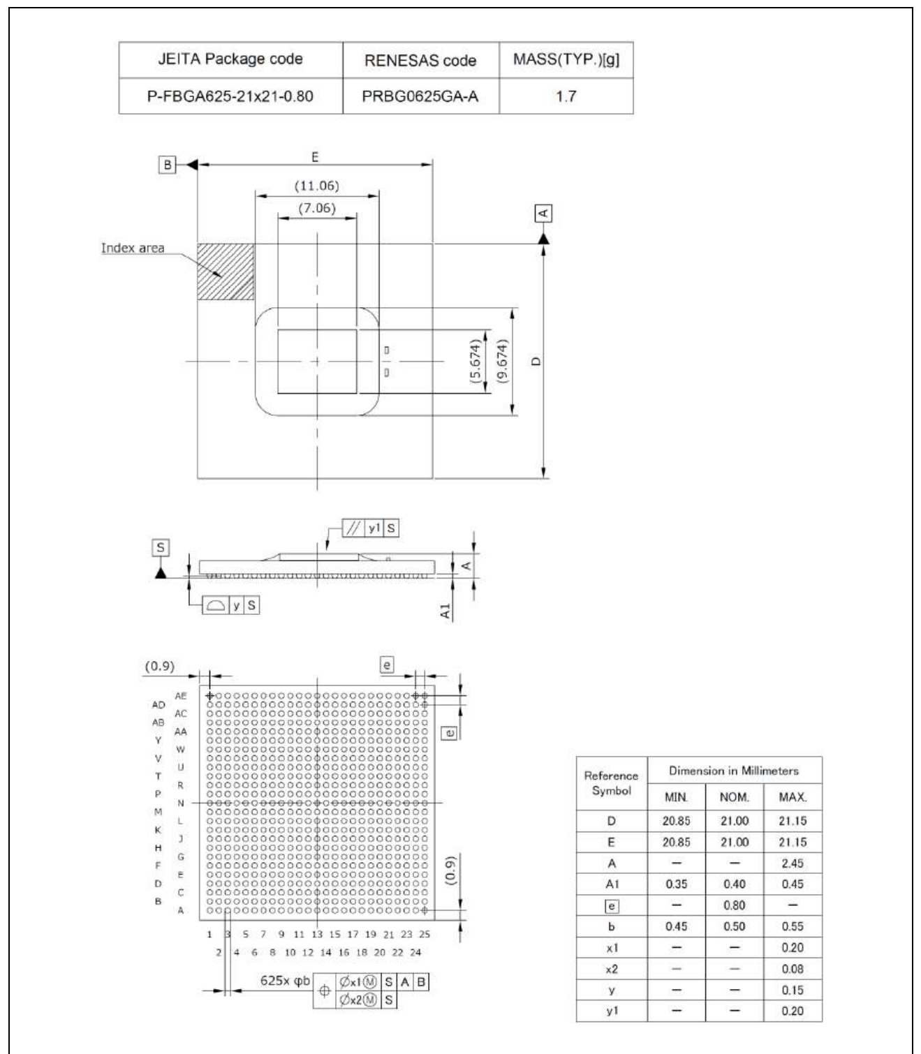
Figure A-2 Package Dimensions (625-pin FCBGA, 21 mm• BGA 0.8 mm pin-pitch)
