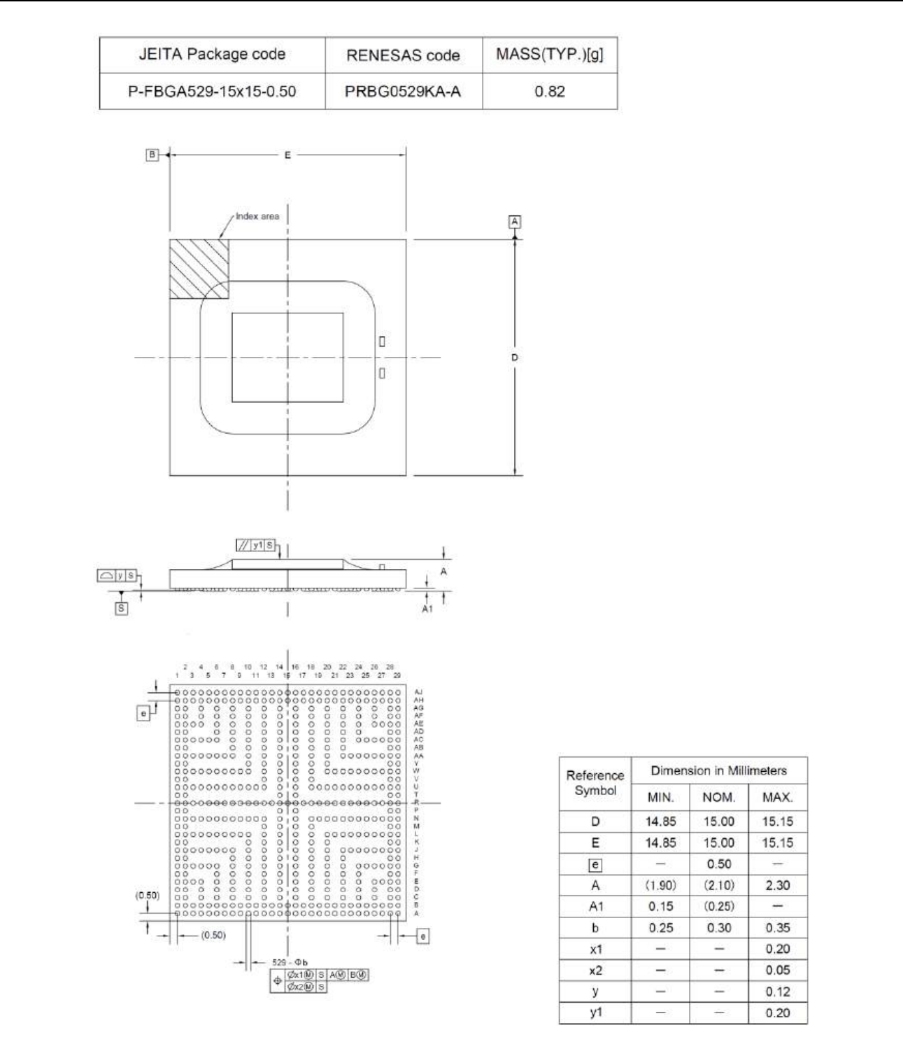
Figure A-1 Package Dimensions (529-pin FCBGA, 15 mm• BGA 0.5 mm pin-pitch)
