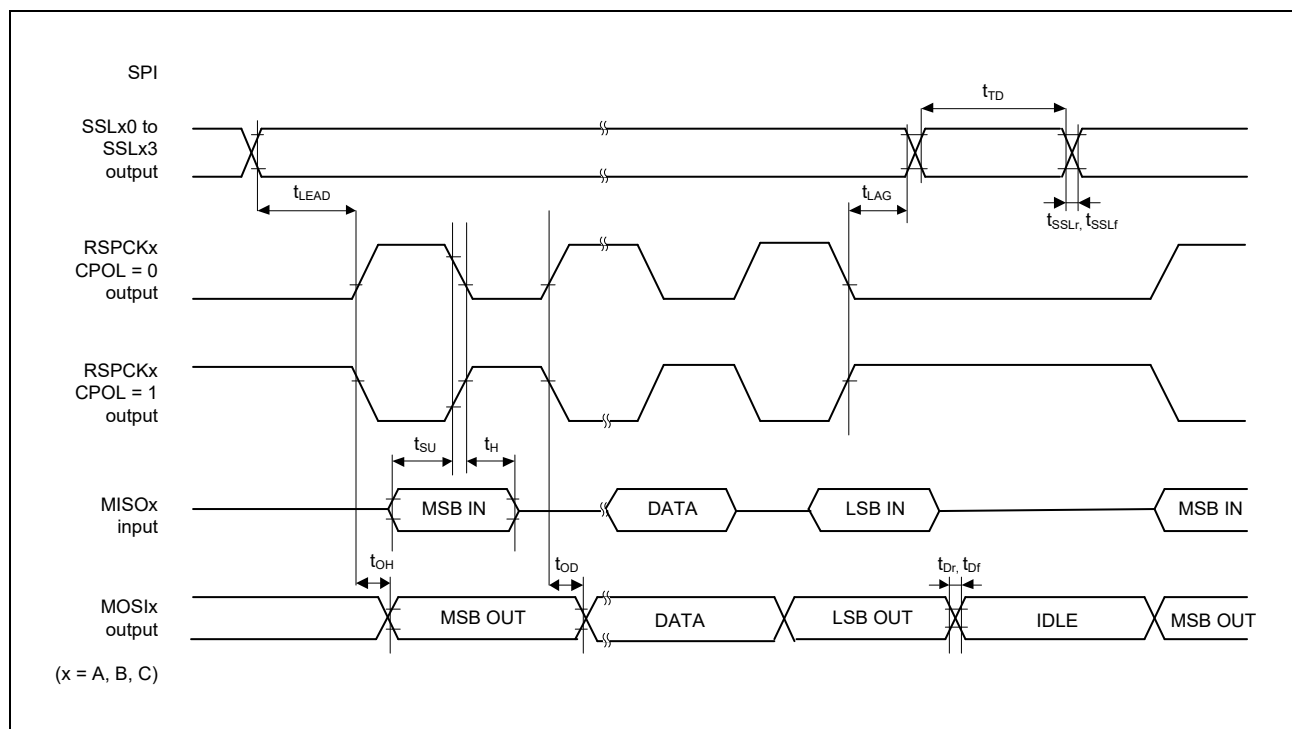
Figure 2.5-30 RSPI Timing (Master, Motorola RSPI, CPHA = 1)
