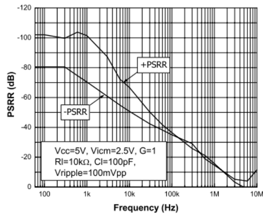
Figure 44. PSSR vs. frequency
