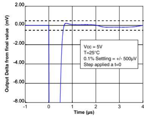
Figure 39. Settling time negative step (2 V to 0 V)
