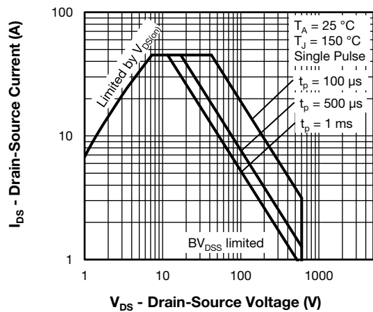
Fig. 28 - MOSFET Safe Operating Area
