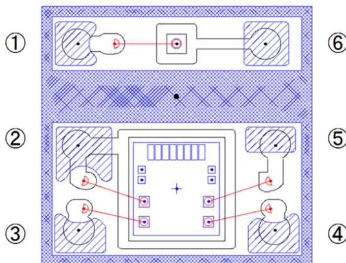
Pin Configuration
