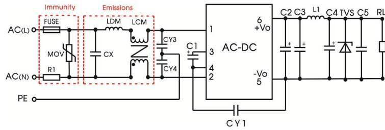
Application circuit 5
