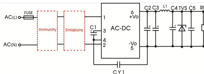
LS series additional circuits design reference
