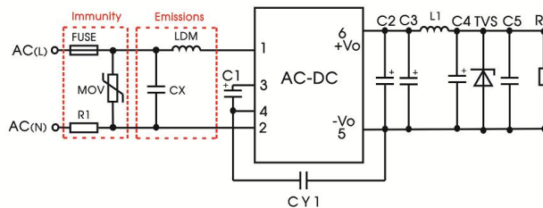
Application circuit 4
