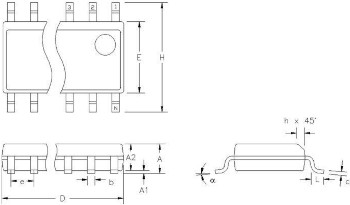
Figure 7 : SOIC8 Package Dimensions [inches]
