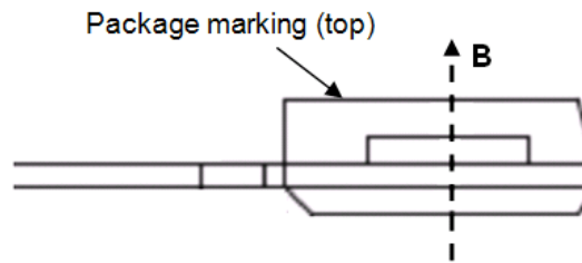
Figure 9: VA/SIP 4L Package. Sensor's active measurement direction
