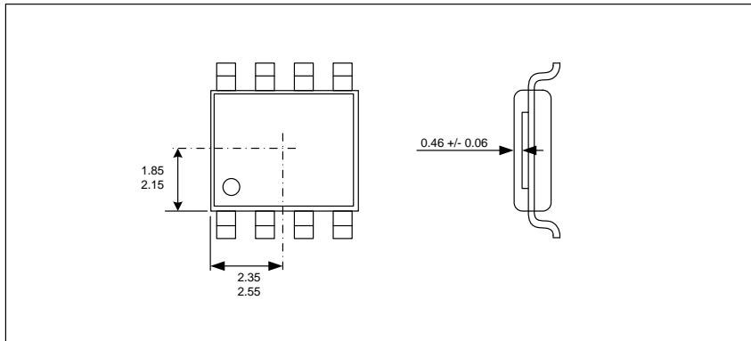
Figure 8: Hall plate position
