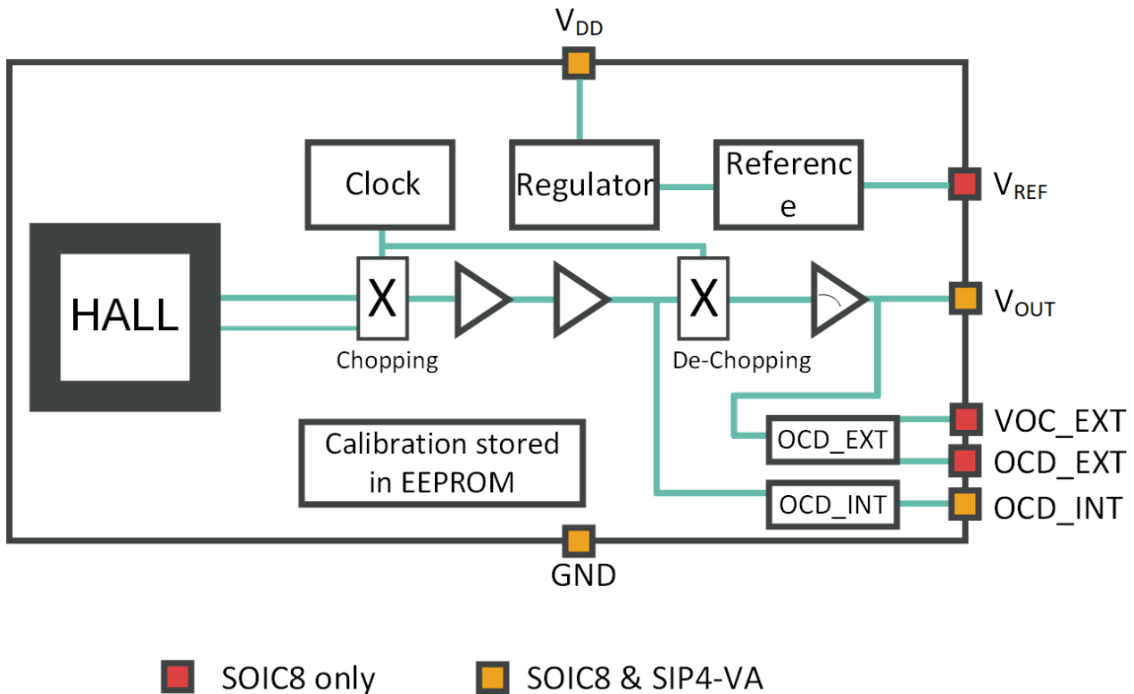
Figure 3 Functional Diagram
