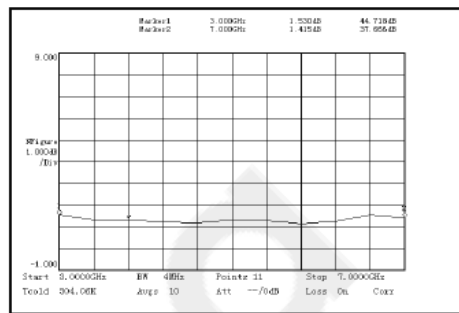
Noise Figure(3-7GHz)
