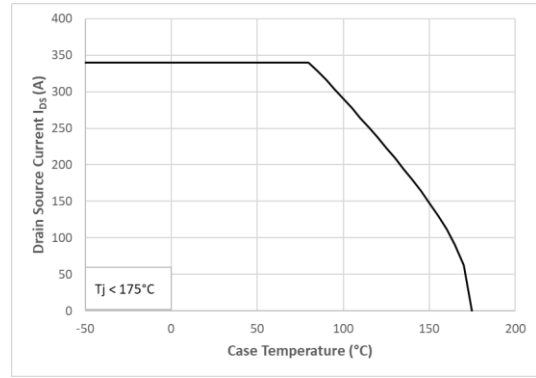
Figure 18: Continuous Drain Current Derating vs Case temperature
