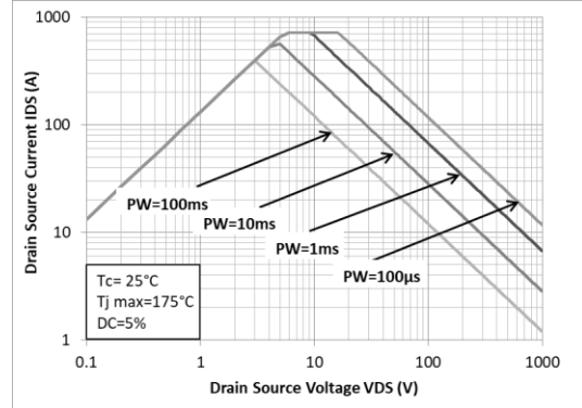
Figure 16: Forward Bias Safe Operating Area (FBSOA)
