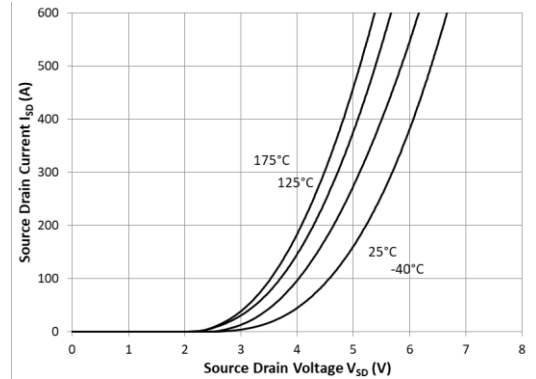
Figure 6: 3rd quadrant characteristics ( V_{GS}=-3V , t_p < 200\mu s ) 7
