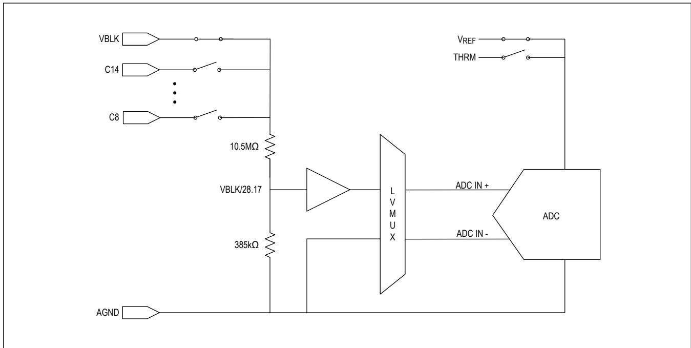
Figure 8. Block-Measurement Path
