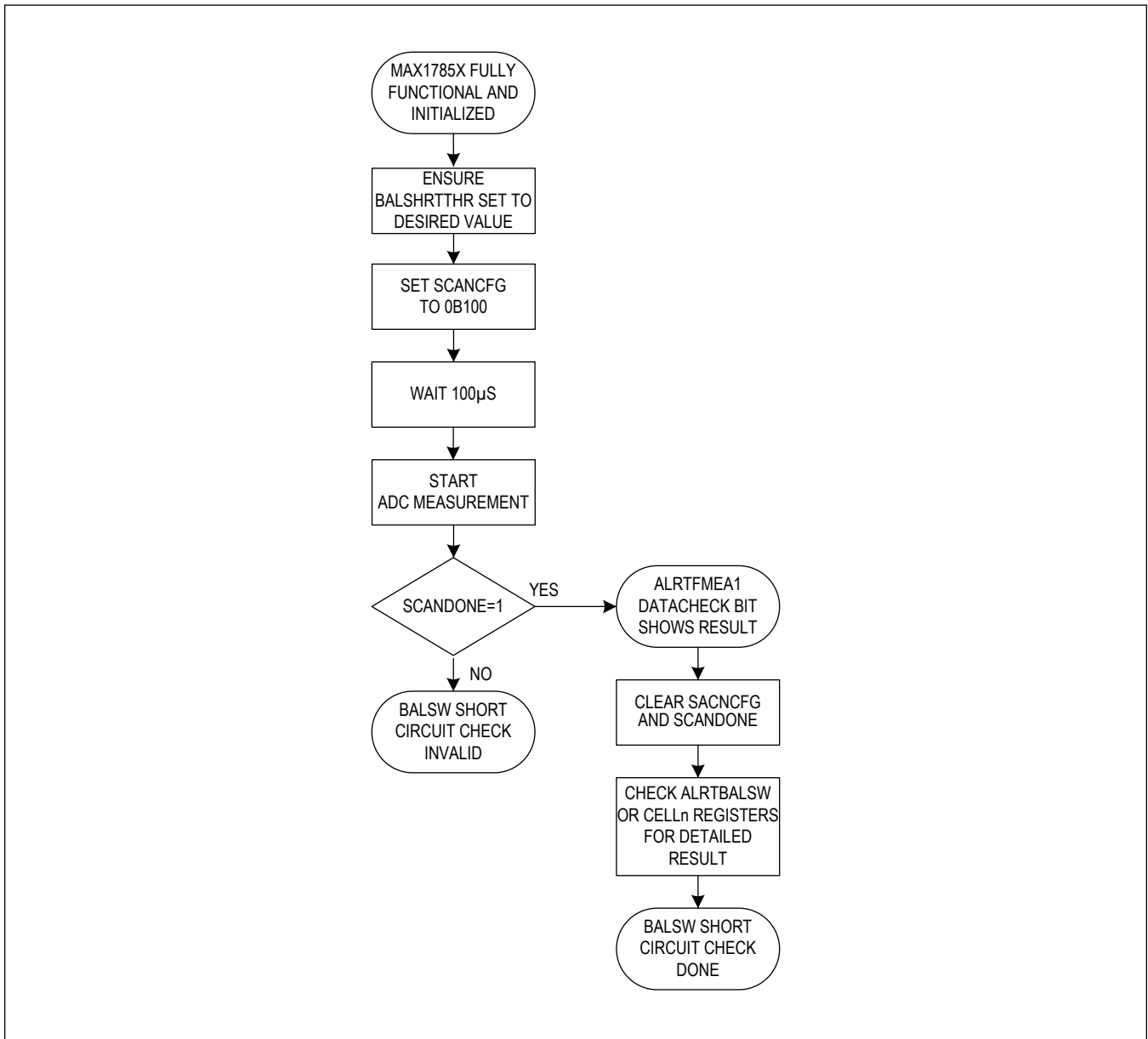
Figure 103. BALS SW Short Diagnostic Chart
