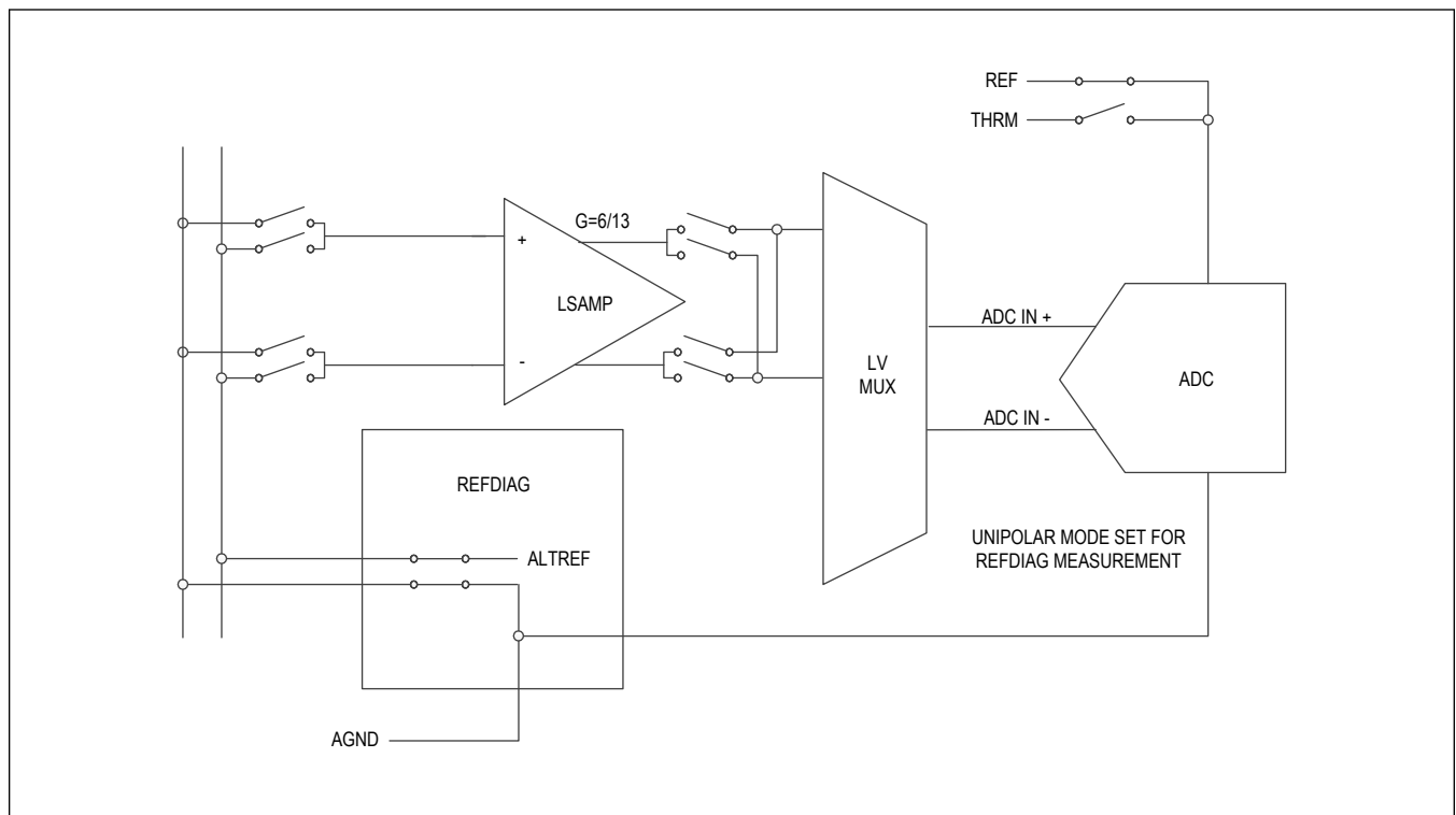
Figure 91. ALTREF Diagnostic
