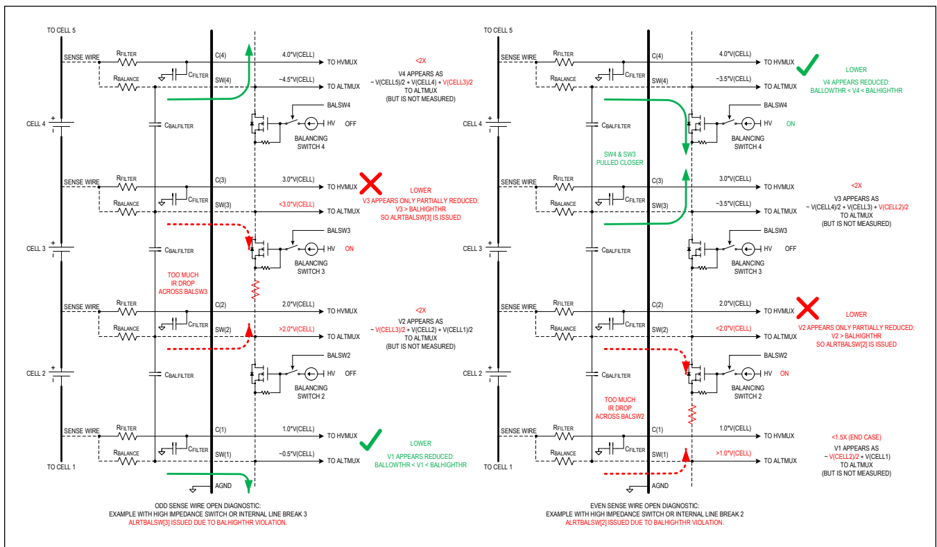
Figure 110. Cell Sense-Wire Open-Diagnostic Operations - Example with Broken BALS or Internal Trace
