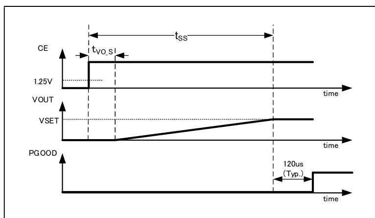
Soft-start Sequence
