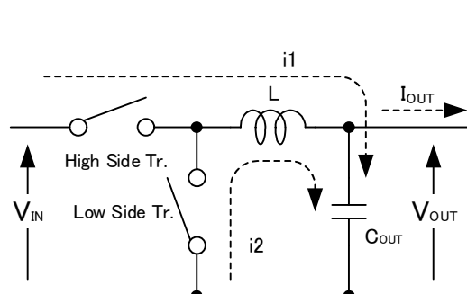
Basic Circuit
