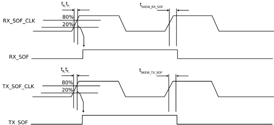
FIGURE 7-9: SOF INDICATION TIMING
