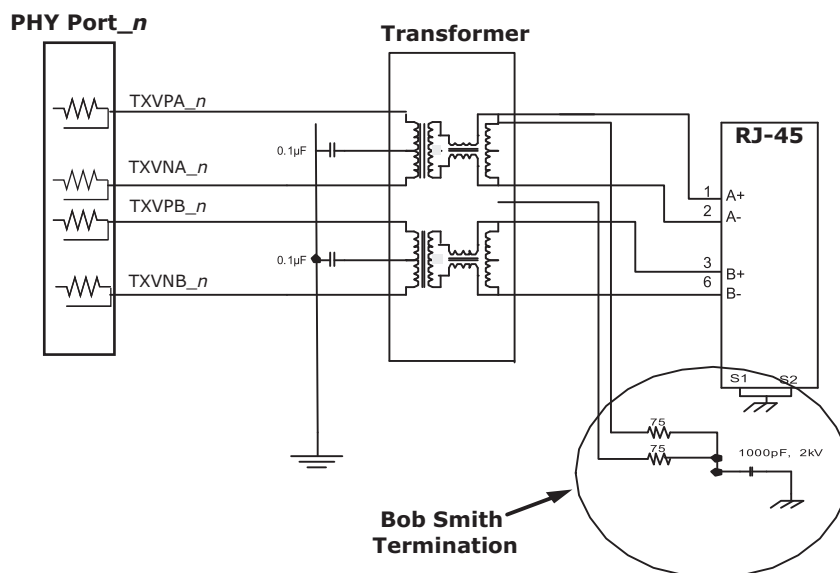
FIGURE 4-6: CAT5 MEDIA INTERFACE
