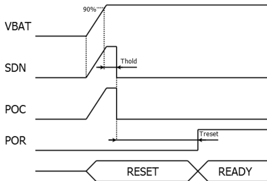
Figure 7. Start-up phase
