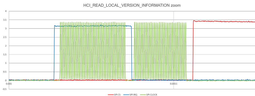
Figure 21. HCI_READ_LOCAL_VERSION_INFORMATION SPI waveform zoom
