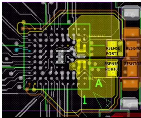
Figure 19. Rsense Resistor Placement (Top Layer)
